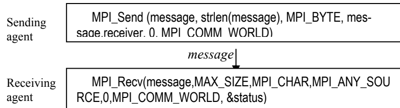
Fig. 9. Flow Chart of Message Communication
