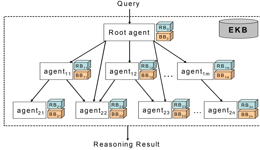
Fig. 1. Architecture of MASAQ
