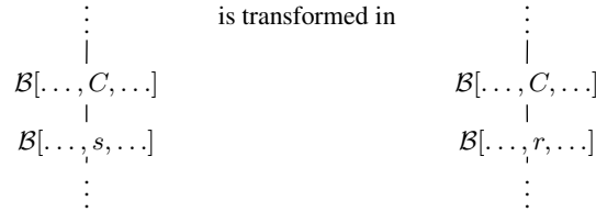
Fig. 1. Updating a branch with a current value.
