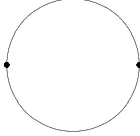
Figure 1: M_6 : the smallest SR-polyhedron, with six elements: two vertices, two edges, two faces
